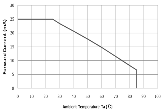
Maximum Forward Current VS. Ambient temperature
