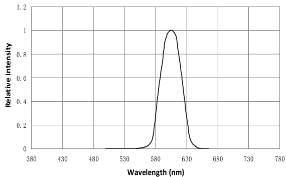
Spectrum Distribution (Ta=25°C)
