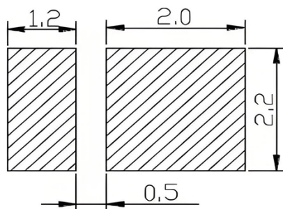
推荐焊盘 Recommended Soldering Pad
