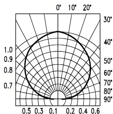
Fig.6 Spatial Distribution
