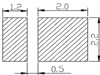
推荐焊盘 Recommended Soldering Pad
