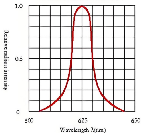
光谱分布曲线 Relative Intensity Vs. Wavelength
