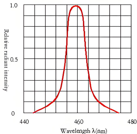
光谱分布曲线 Relative Intensity Vs. Wavelength
