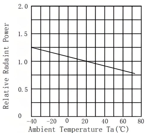
Radiant Power Vs. Ambient Temperature
