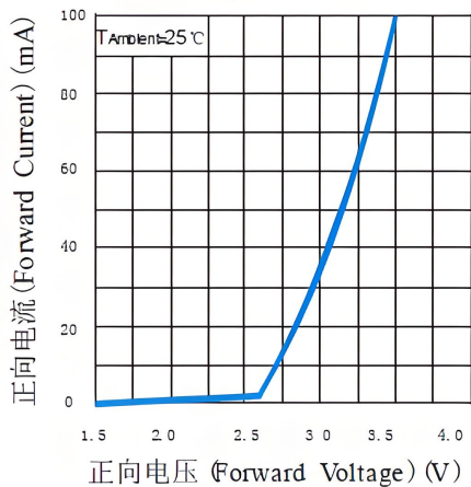
伏安特性 Volt-Ampere Characteristics
