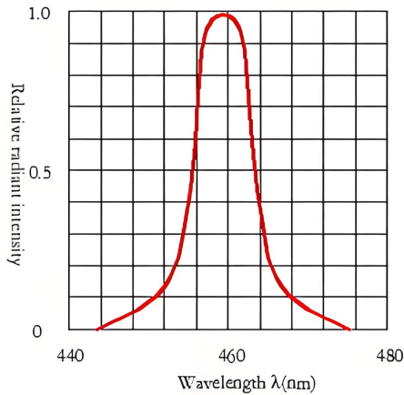
光谱分布曲线 Relative Intensity Vs. Wavelength
