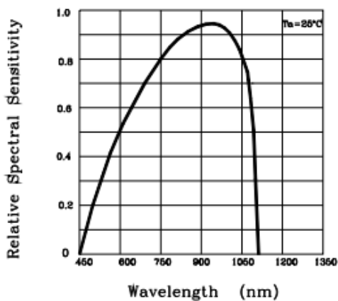
Fig. 5 Spectral Sensitivity
