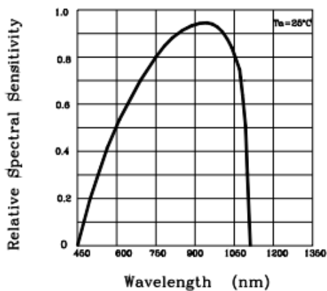
Fig. 5 Spectral Sensitivity
